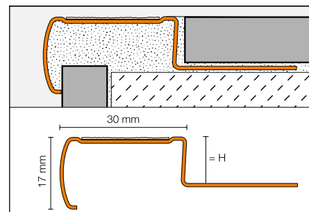
Schlüter-TREP-G-S /-GL-S
